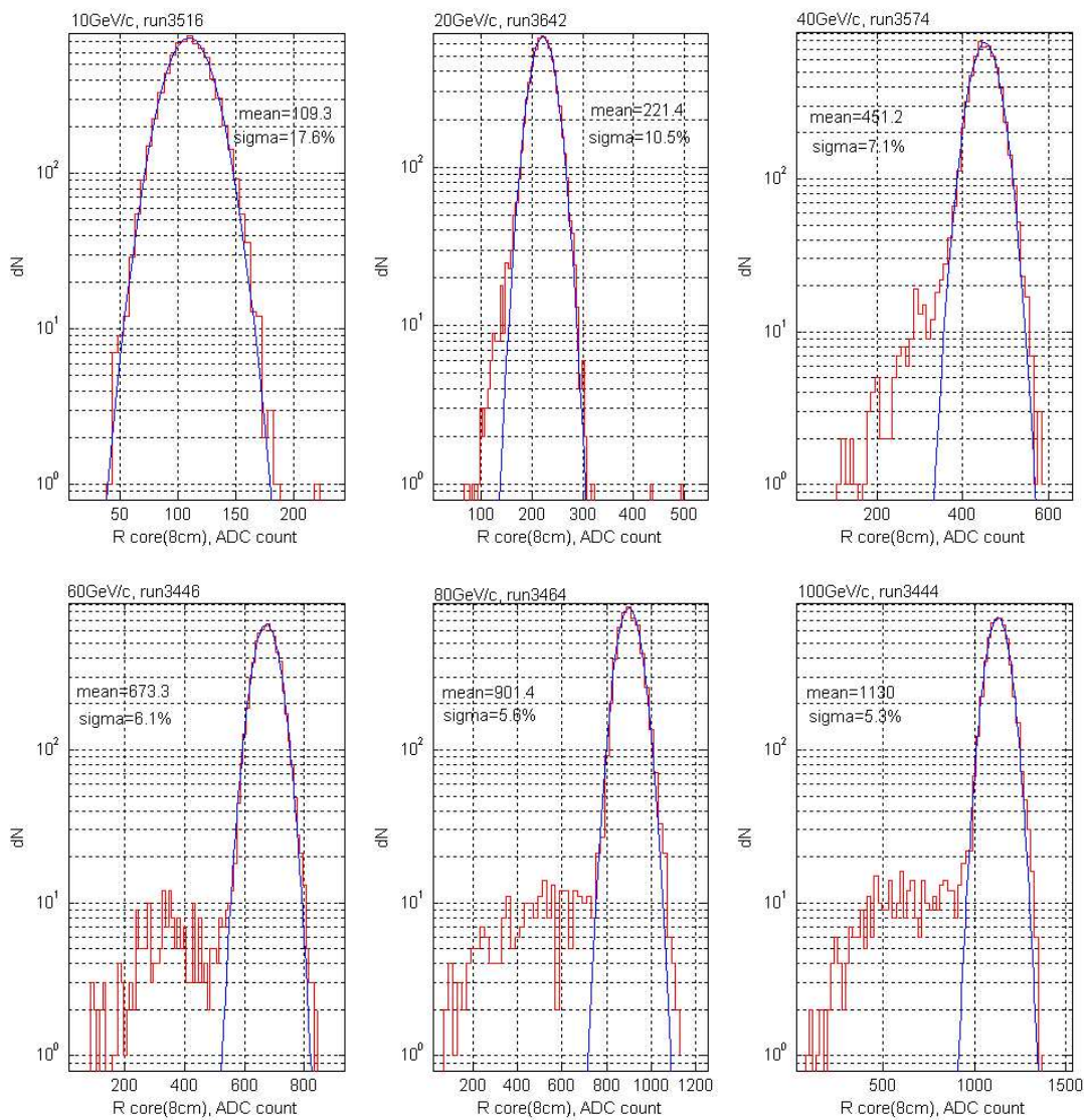
Fig.1. Electron response
