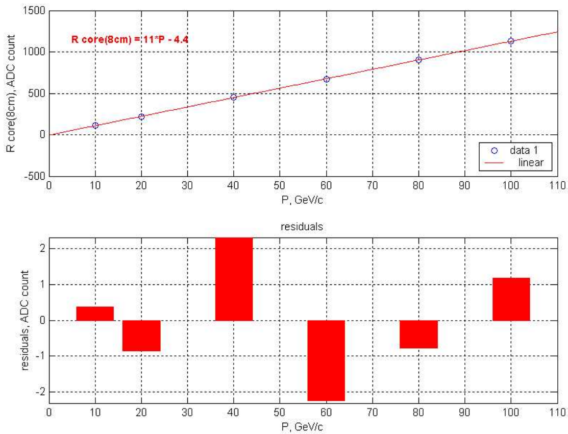
Fig.2. Response linearity for electrons
