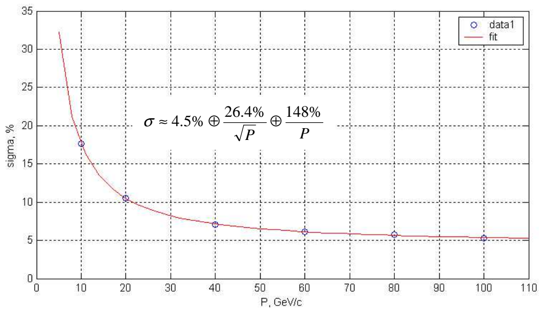
Fig.3. Sigma vs. P for electrons
