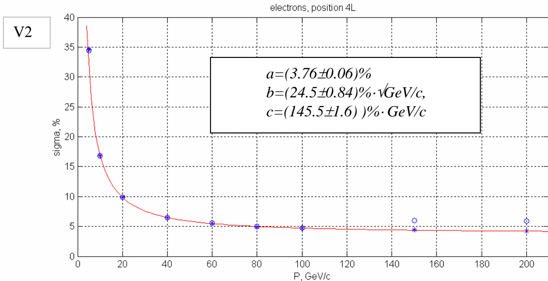
Figure 3: FCAL1 energy resolution for electrons in position 4L, with r_{\text{core}}=8\text{cm} , for the definition V2 of norm_m . The points are: \circ – calibration off, * – calibration on. The line shows the fit with the function \sigma = a \oplus \frac{b}{\sqrt{P}} \oplus \frac{c}{P} ( P in \text{GeV}/c ). With the alternative definition V1, the data points and the fit are indistinguishable from V2.
