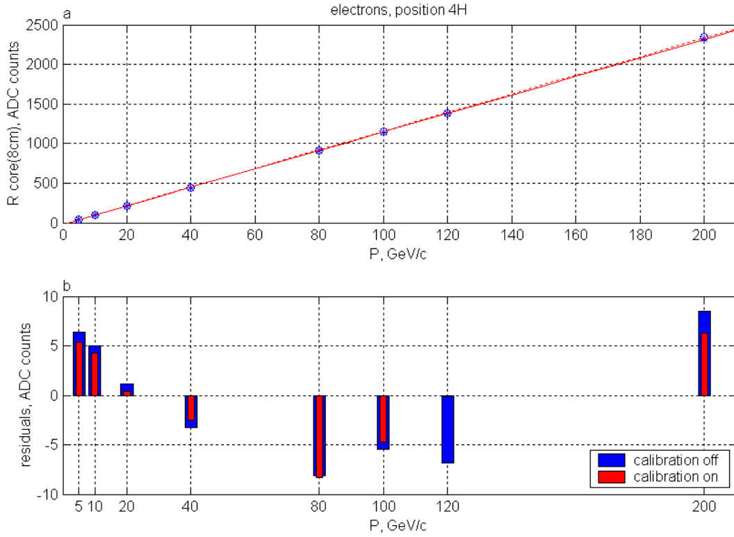
Figure 2: The linearity plot for electrons, position 4H. The fit parameters: calibration off - R = 11.77 \cdot P - 20.52 , calibration on - R = 11.67 \cdot P - 19.29 , where R is the response in ADC counts, P – the beam momentum in \text{GeV}/c .
